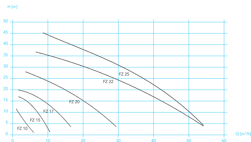
Characteristic curves of the Fristam series FZ; n = 1,450 min -1
