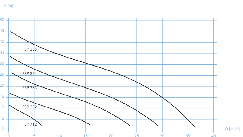
Characteristic curves of the Fristam series FSP
